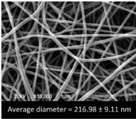
SEM images of PA 6/66 electrospun nanofibers
